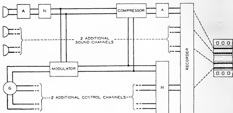
FIG. 3. Block schematic
